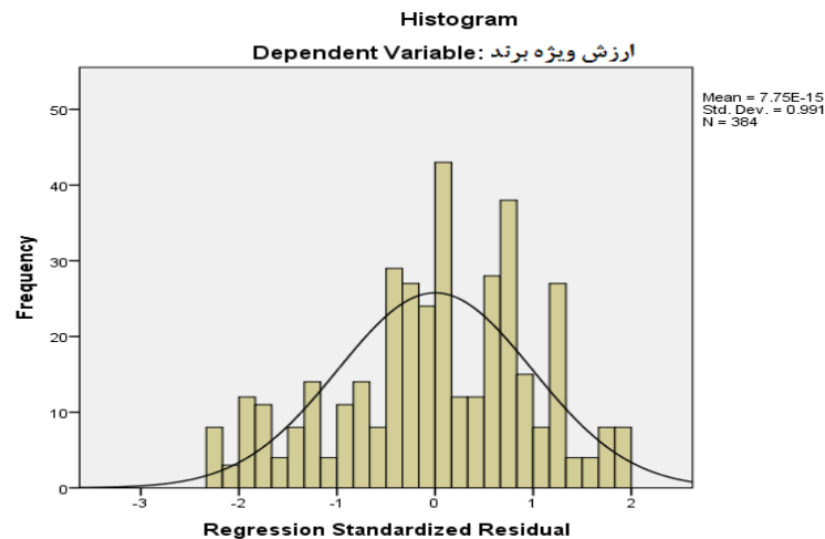
Figure 1: comparison of the distribution of errors with normal distribution
